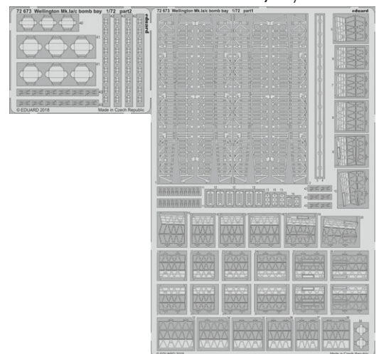
72673 Wellington Mk.Ia/c bomb bay 1/72 Airfix
