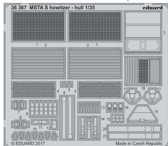
36367 MSTA S howitzer - hull 1/35 Zvezda
