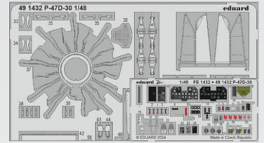
491432 P-47D-30 1/48 MINIART (2 parts)
