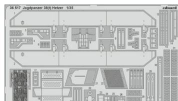
36517 Jagdpanzer 38(t) Hetzer 1/35 Takom (1 part)
