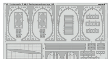
481133 Lancaster B Mk.III Dambuster undercarriage 1/48 HKM (1 part)
