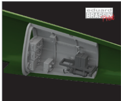
672318 Bf 109F radio compartment PRINT 1/72 Eduard
