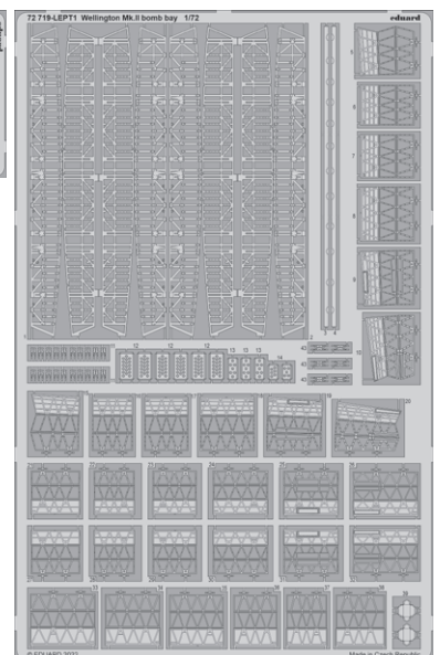
72719 Wellington Mk.II bomb bay 1/72 Airfix
