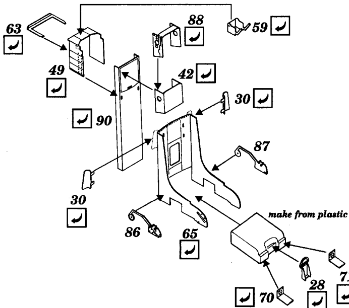
SK-2 EJECTION SEAT
