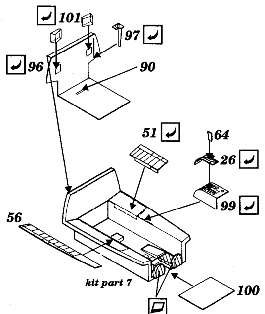
MB EJECTION SEAT
