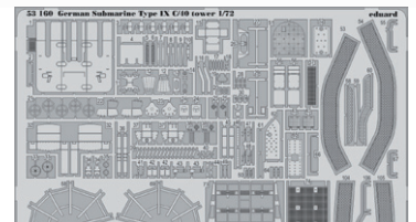
53160 German Submarine Type IX C/40 tower 1/72 Revell (1 part)
