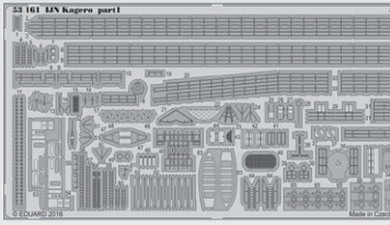
53161 IJN Kagero pt.1 1/350 Tamiya (1 part)
