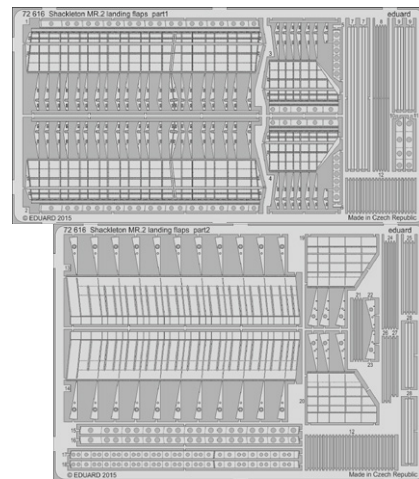
72616 Shackleton MR.2 landing flaps 1/72 Airfix
