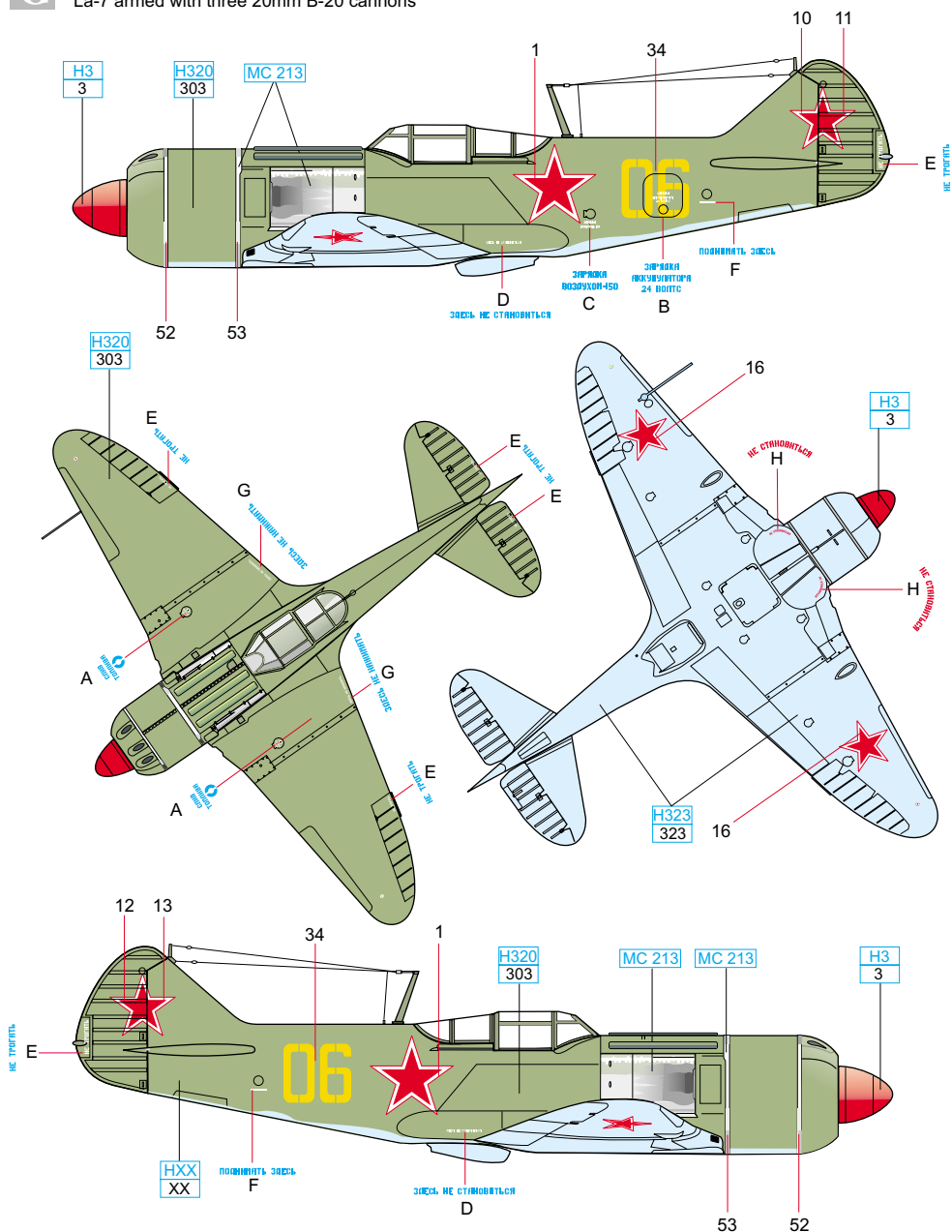
La-7 armed with three 20mm B-20 cannons
